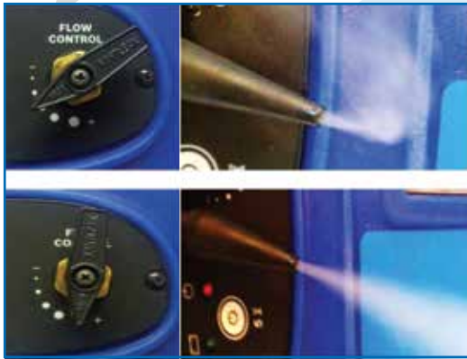
Adjust the Flow Control for finer adjustment to find even smaller leaks
